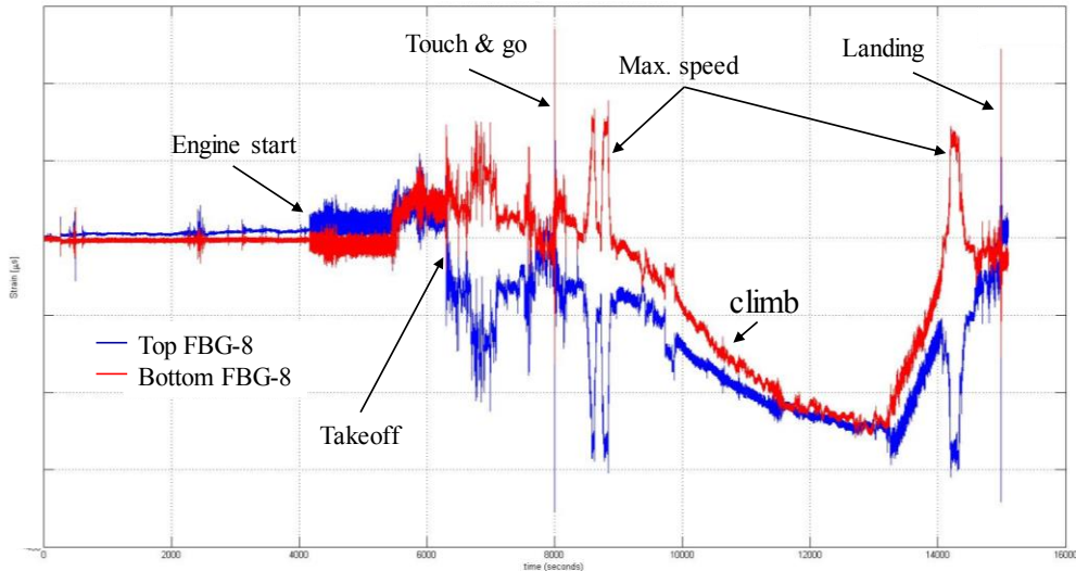
Figure 5: Typical FBG readings of boom mounted FBG (Top and bottom sensors)
