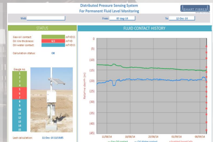
Example SmartSoft visualisation of reducing oil level in wellbore
